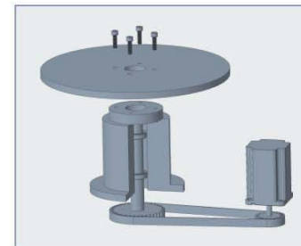
皮带轮+机构部件再连接电机 Pulley + mechanism parts and then connected to the motor
