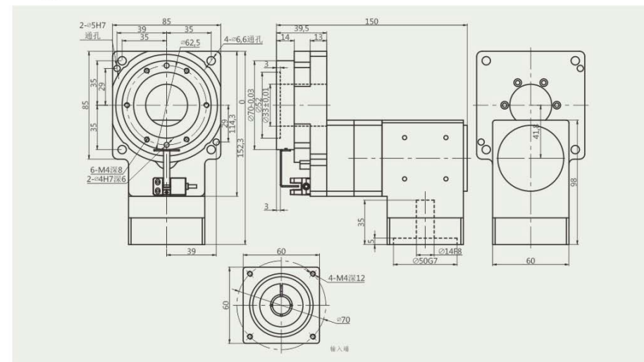
HRT85RL-10 配400W伺服接口 for 400W Servo Interface
