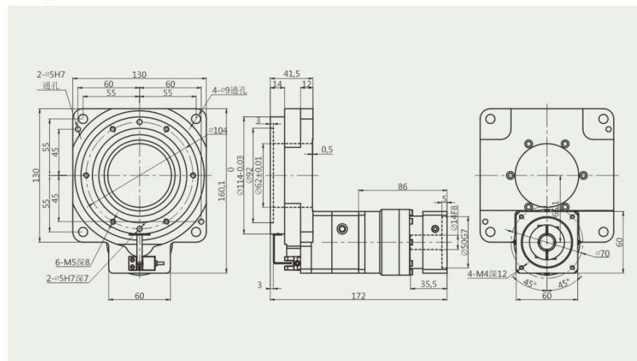
HRT130JS-30 配400W伺服接口 for 400W Servo Interface
