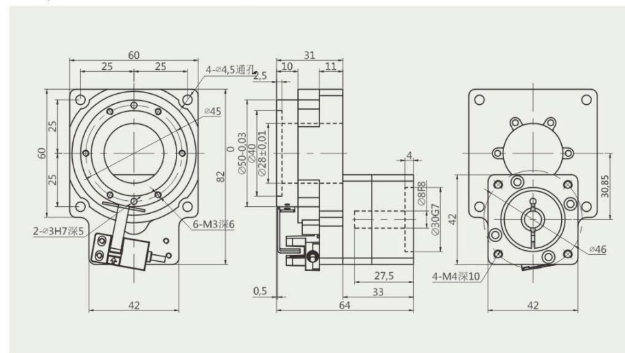
HRT62-10 配100W伺服接口 for 100W Servo Interface
