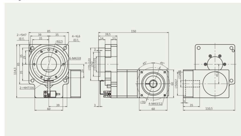
HRT85RY-10 配400W伺服接口 for 400W Servo Interface
