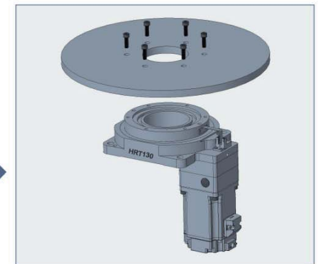
中空旋转平台直接连电机 The hollow rotating platform is directly connected to the motor
