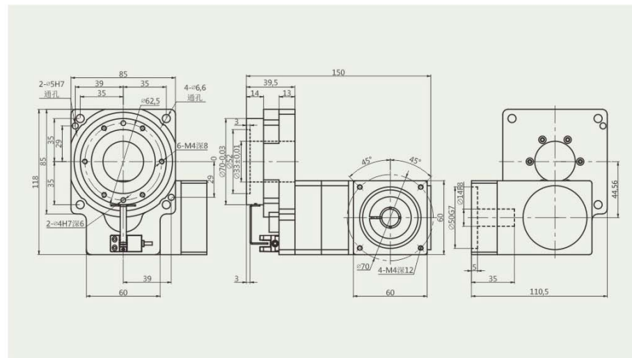
HRT85RY-5 配400W伺服接口 for 400W Servo Interface
