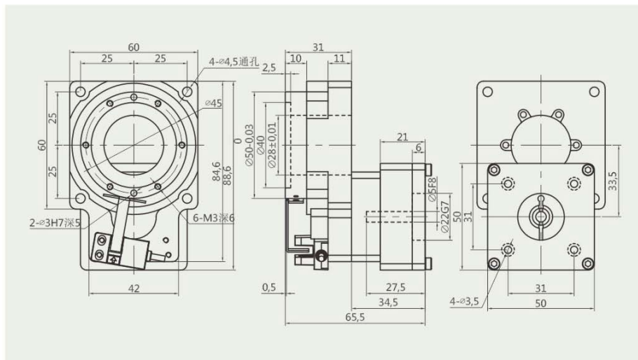
HRT62-5 配42步进接口 for 42 Stepper Interface
