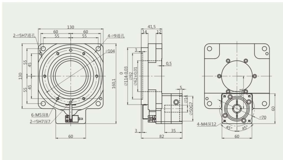
HRT130-10 (18) 配400W伺服接口 for 400W Servo Interface
