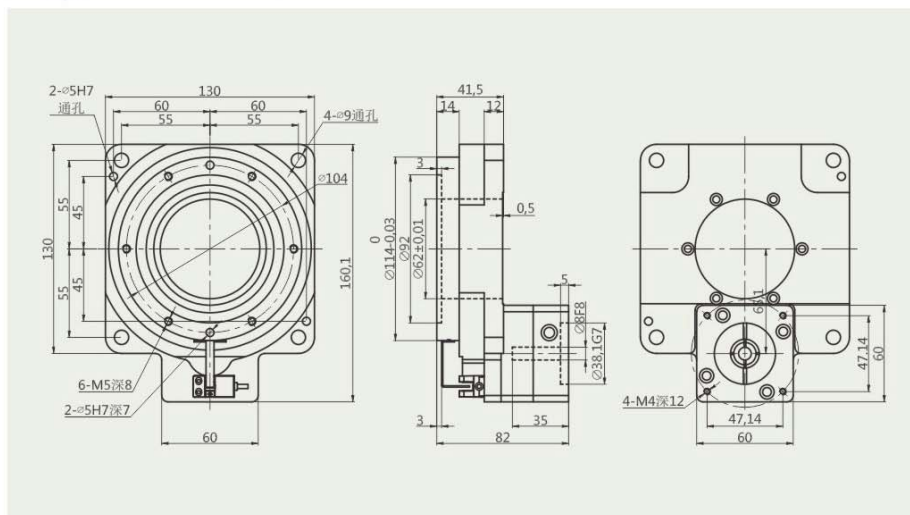
HRT130-10 (18) 配57步进接口 for 57 Stepper Interface
