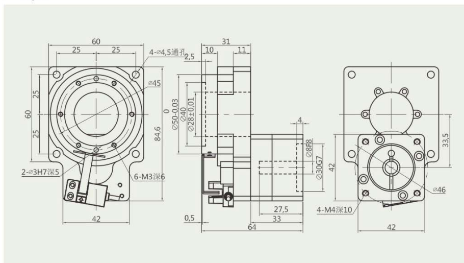
HRT62-5 配100W伺服接口 for 100W Servo Interface
