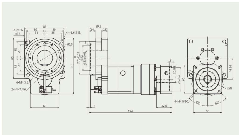
HRT85JS-15 配400W伺服接口 for 400W Servo Interface
