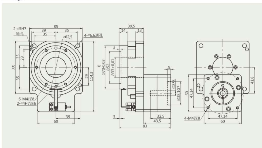
HRT85-10 配57步进接口 for 57 Stepper Interface
